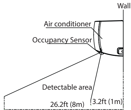
Fig. 17 —Occupancy Sensor Detectable Range
